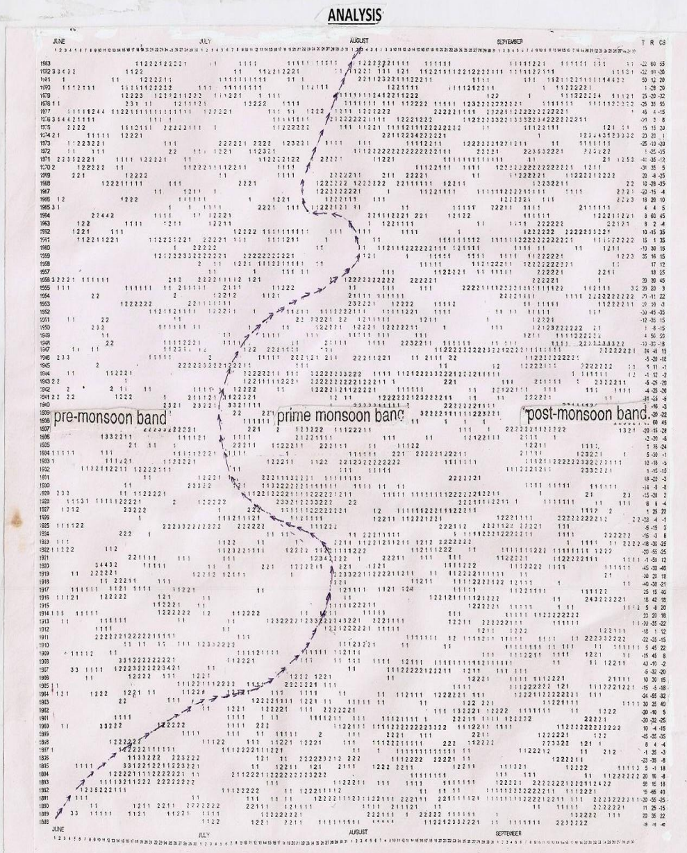
path of the systematic cycle of the Indian Monsoon.
